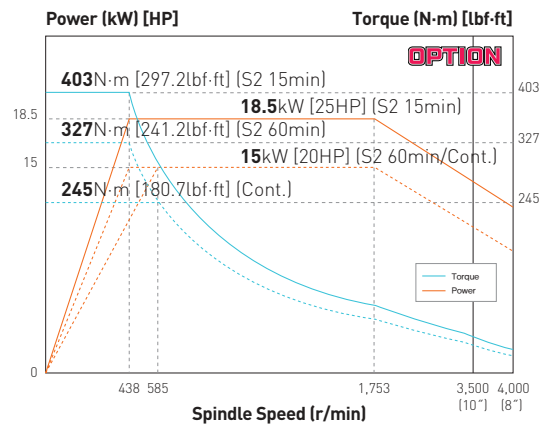
LF2600 II Series 3,500/4,000 rpm (High-Torque)
