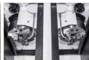
Chuck Coolant (Upper Chuck)
